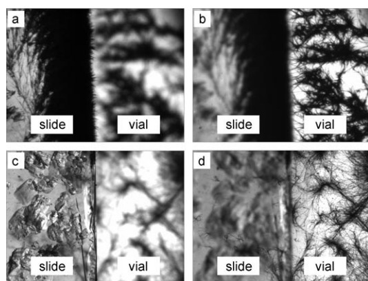
Figure 3. Indomethacin crystal growth by using method 1. Slides functionalized with silane monolayers are on the left side of the images. The right portions of the images show the bottoms of the vials not covered by the slides. a,b) Crystal growth on 5 monolayers with focus on the slide (in a) and on the vial (in b). Notice the predominant growth of \alpha polymorph on both locations. c,d) Crystal growth on 9 monolayers with focus on the slide (c) and on the vial (d). Notice the predominant growth of \gamma polymorph on the slide and \alpha polymorph at the bottom of the vial. See also Figure S7 in the Supporting Information.
